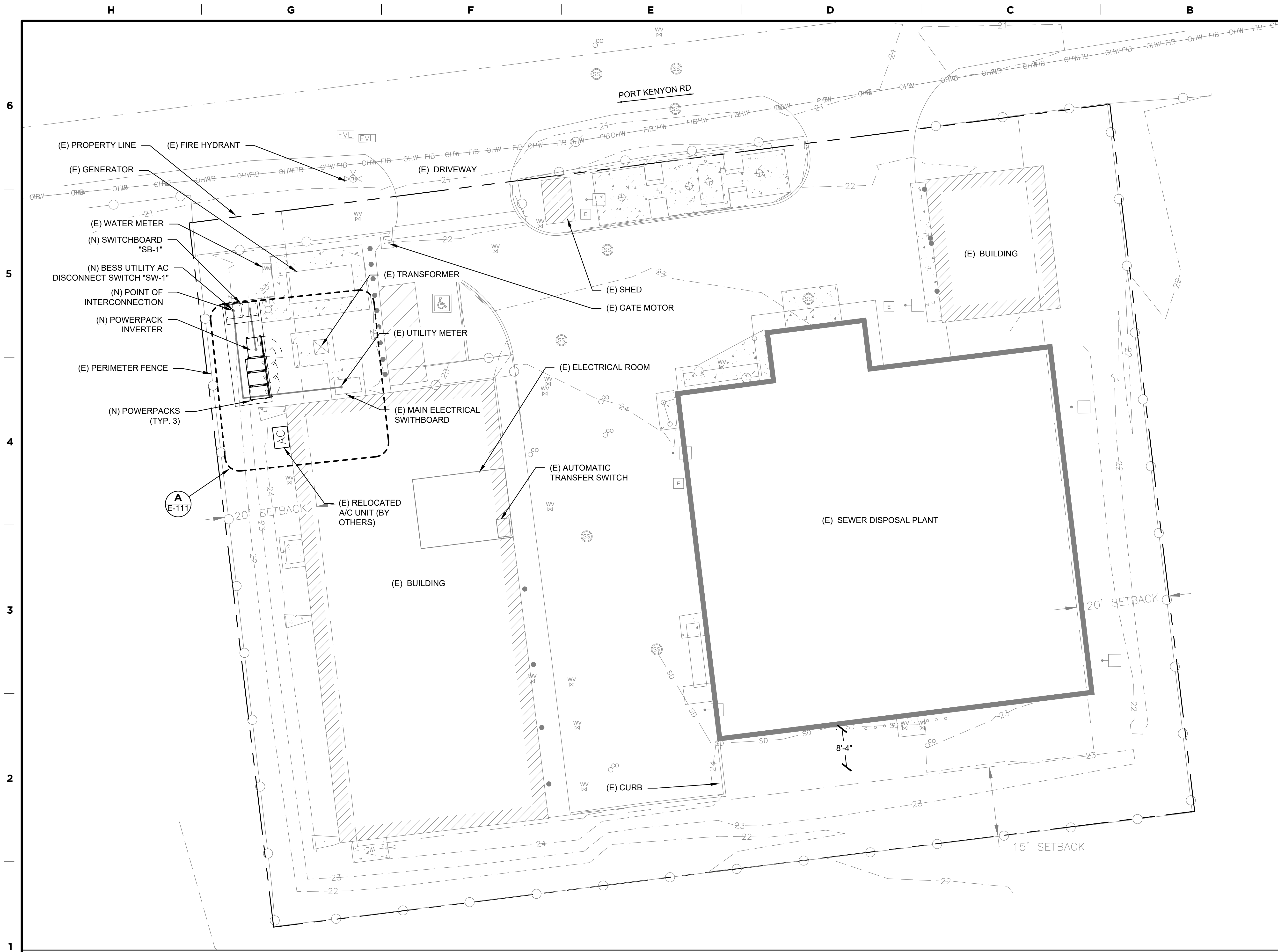
ELECTRICAL SITE PLAN 1" = 10'-0"
