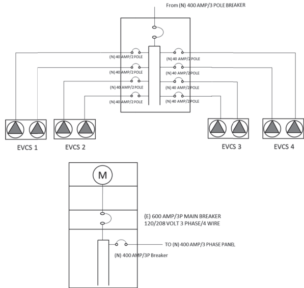
5 C4 ONE LINE DIAGRAM ELEMENTS
