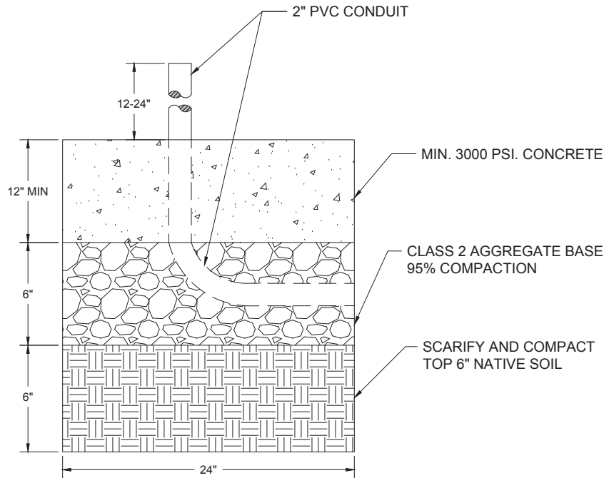
(N) CHARGEPOINT CONCRETE PAD DETAIL
