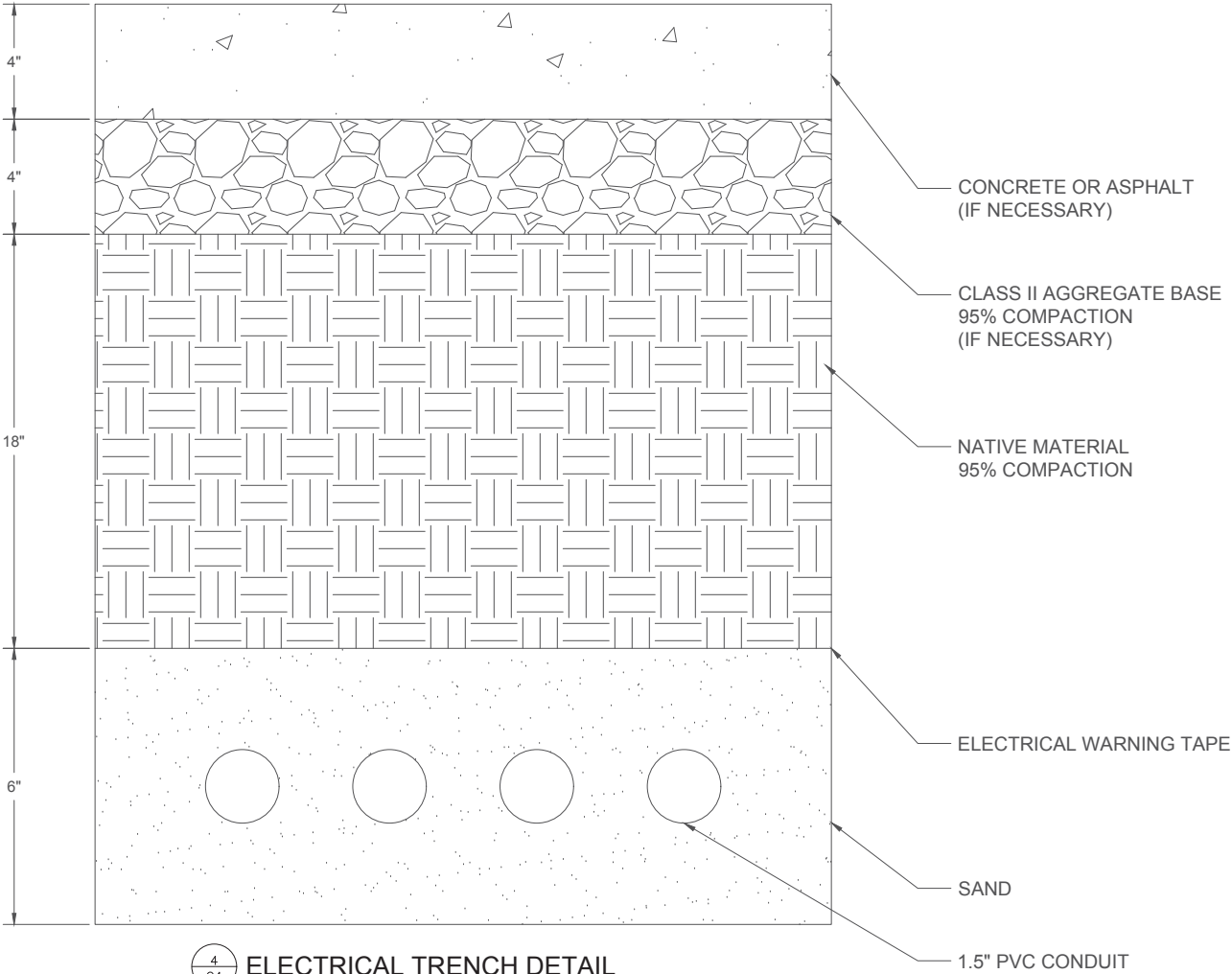
4 C4 ELECTRICAL TRENCH DETAIL
