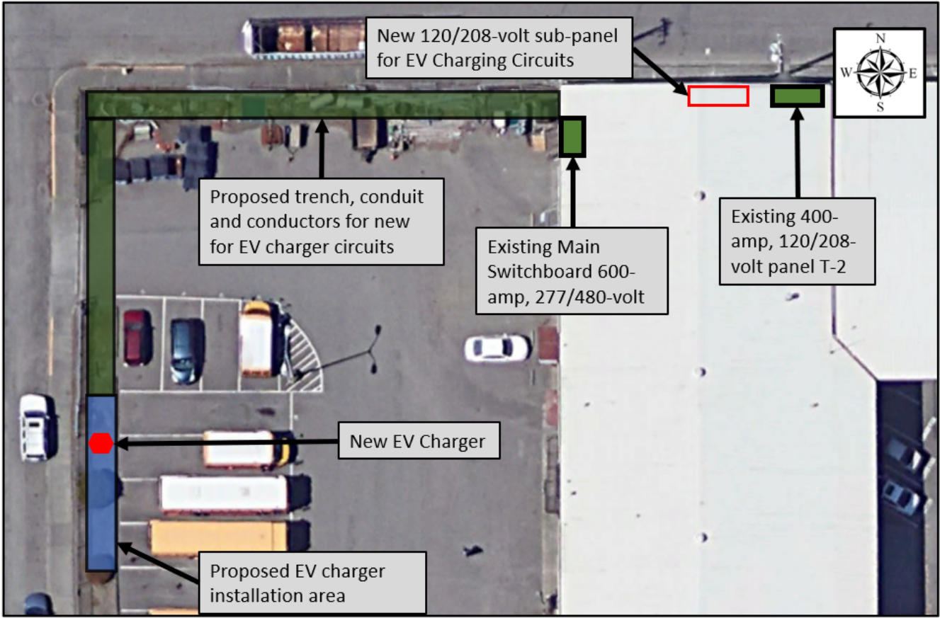
Figure 2 Potential configuration of new electrical infrastructure at ECS's Corporation Yard.
