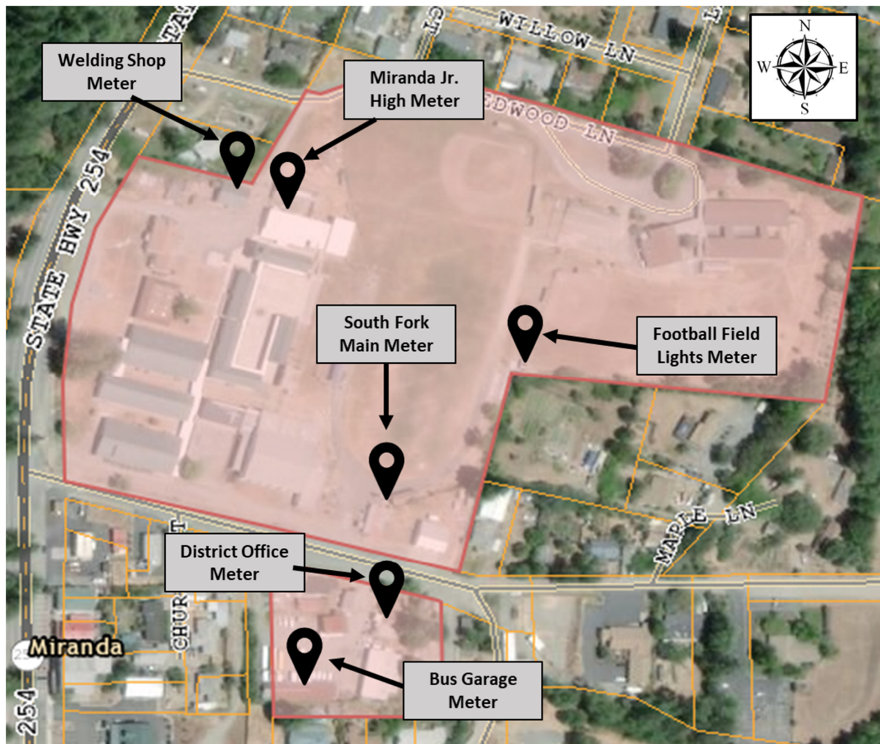
Figure 4 Site map showing South Fork site parcel boundaries and meter locations.
