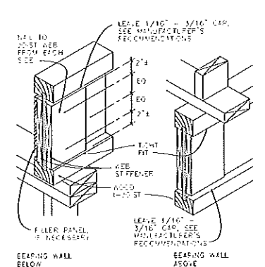
1 JOISTS AT BEARING WALL DETAILS
