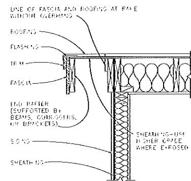
RAKE OVERHANG DETAIL
