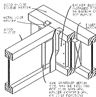
1 JOIST TO 1 JOIST HEADER DETAIL
