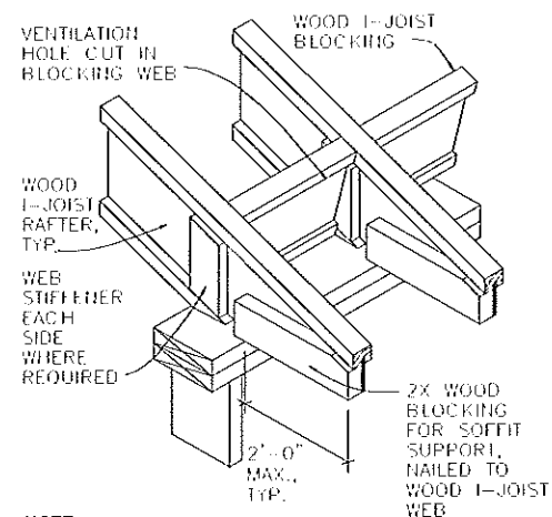
RAKE OVERHANG DETAIL
